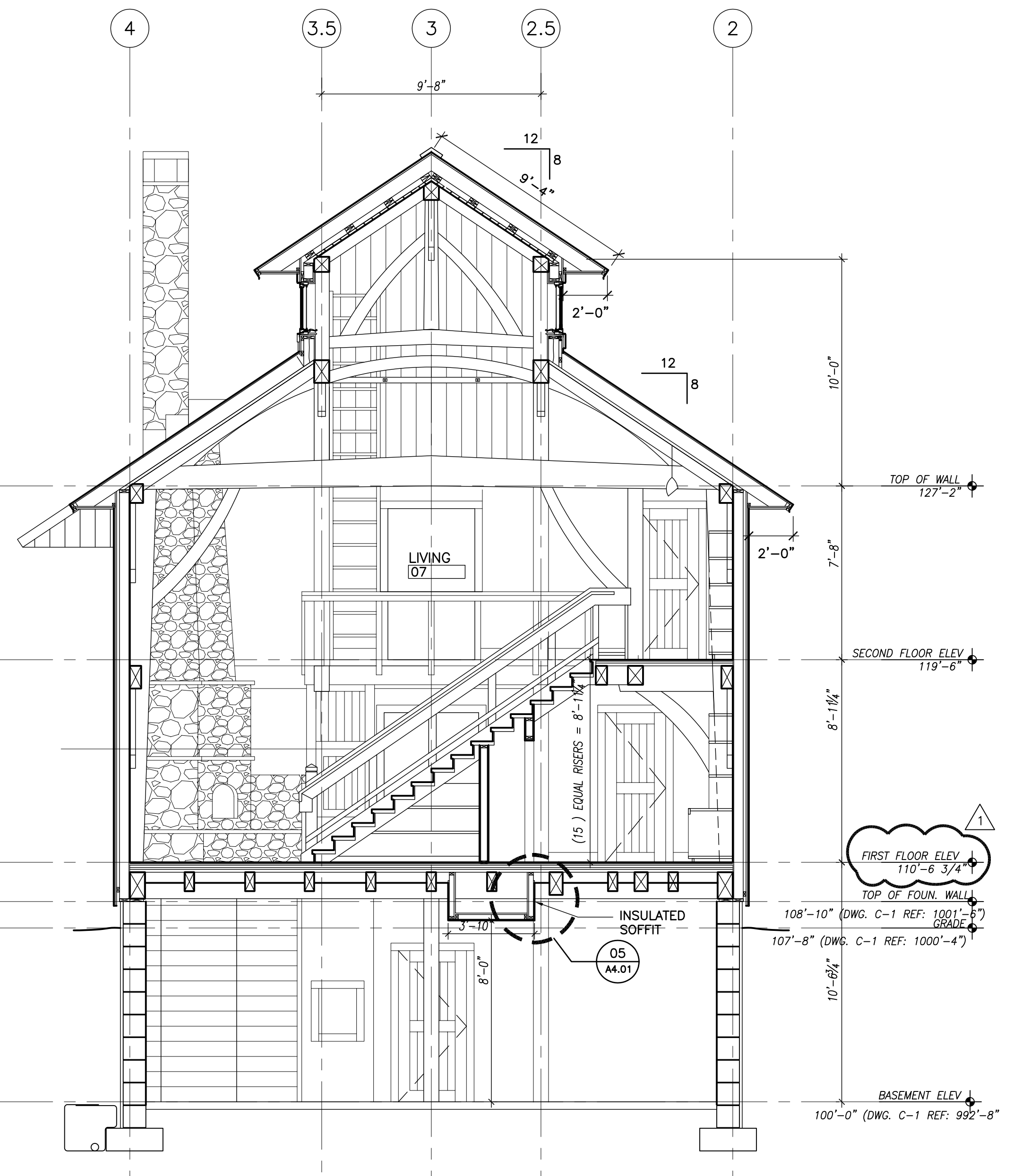
01 BUILDING SECTION SCALE: 1/4" = 1'-0"
