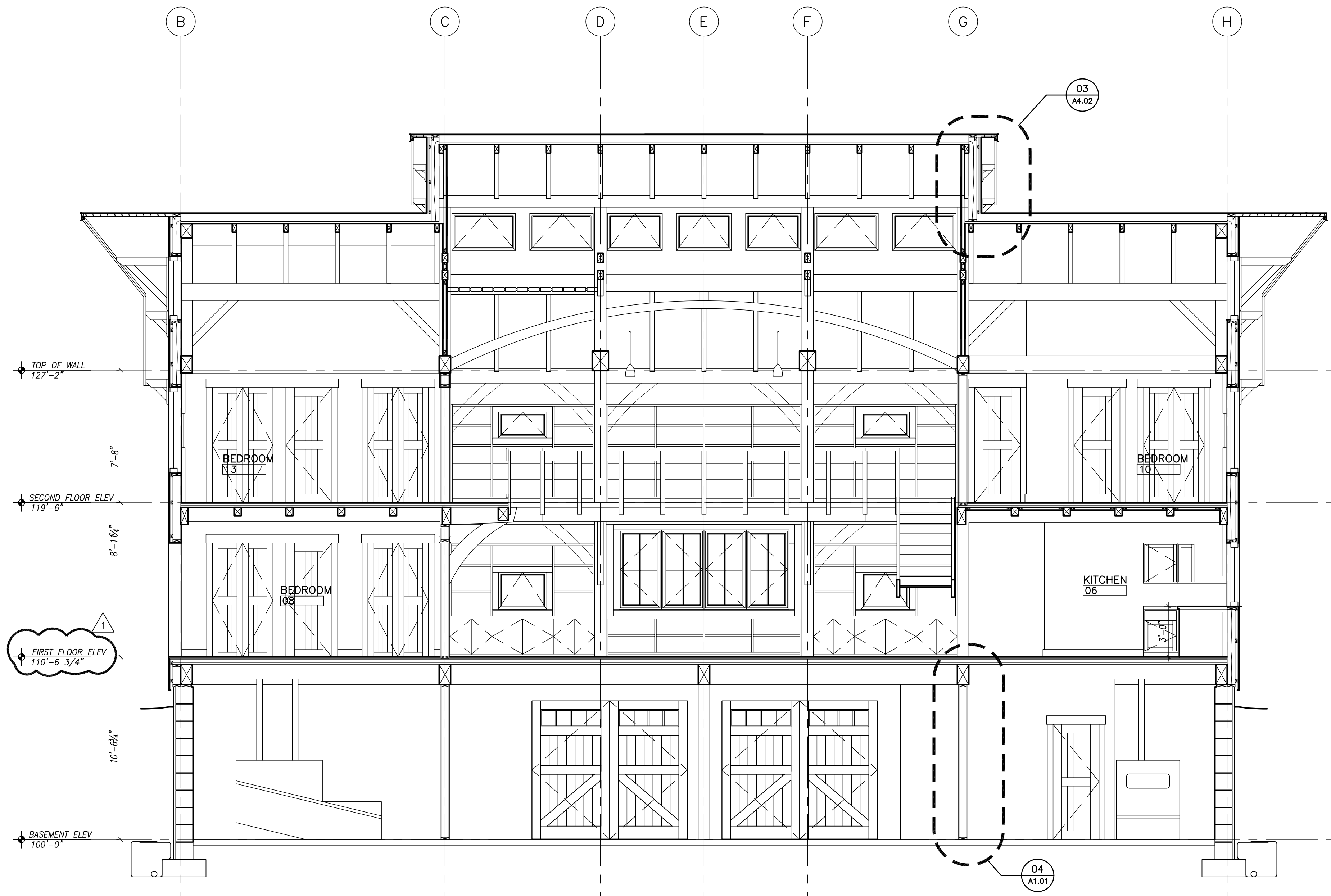
02 BUILDING SECTION SCALE: 1/4" = 1'-0"
