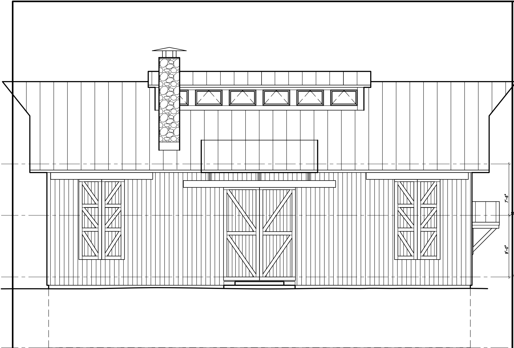
○ SOUTH EAST ELEVATION—OPTION 3 1/8" = 1'-0"
